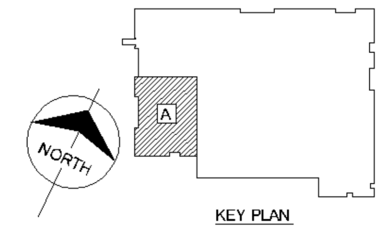
BUILDING 560 ENLARGED FIRST FLOOR PLAN - WASTE & VENT DEMOLITION - AREA A 8' 4' 0' 8' SCALE: 1/8" = 1'-0"
